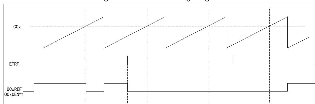
Figure 77 OCxREF Timing Diagram
