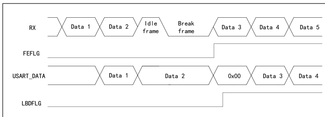
Figure 89 Break Frame Detection in Idle State
