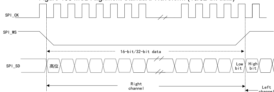
Figure 109 MSB Alignment Standard Waveform (24-bit data)
