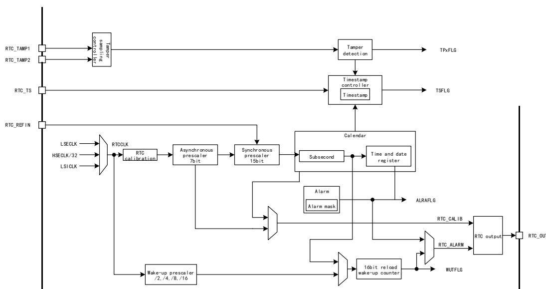
Figure 82 RTC Structure Block Diagram
