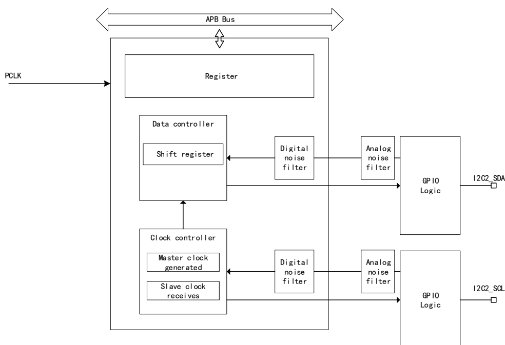
Figure 96 I2C2 Function Structure Diagram
