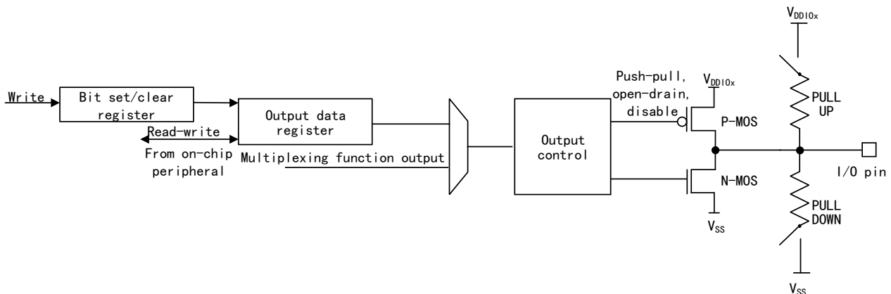
Figure 19 I/O Structure in Output Mode
